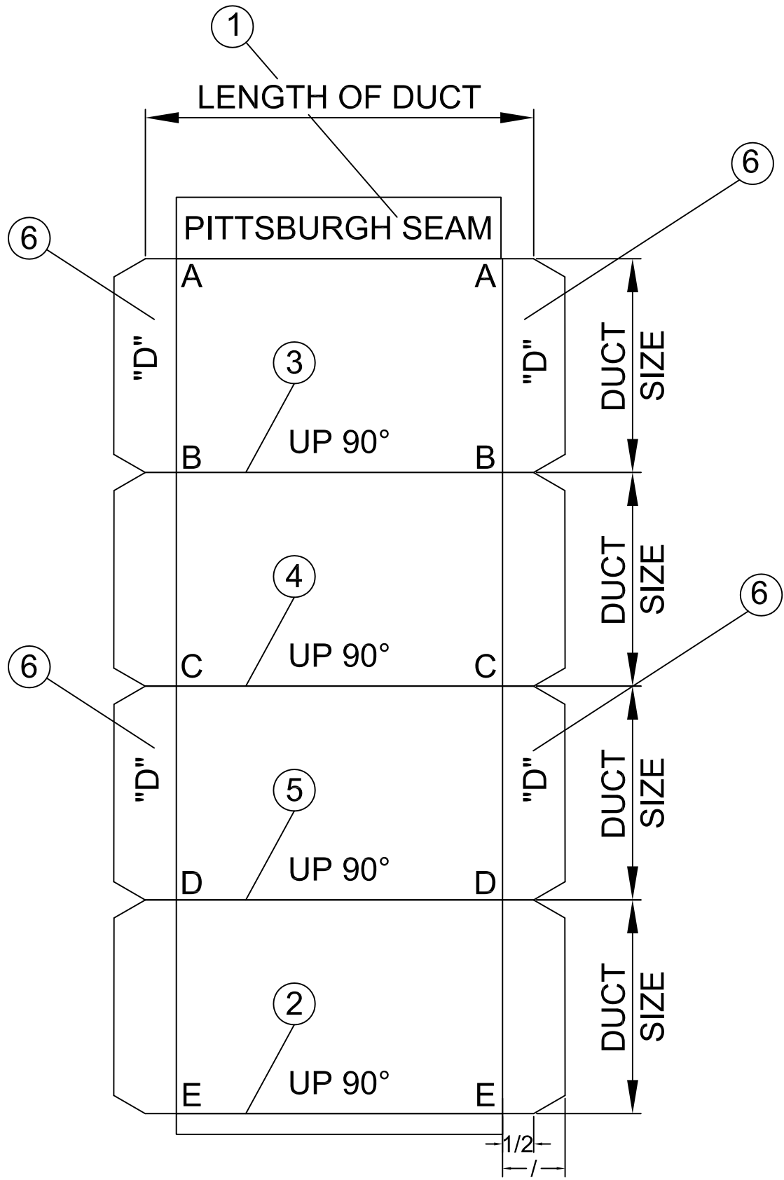
DUCT PATTERN
